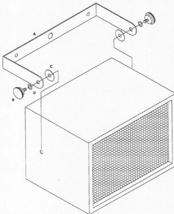
FIGURE 1 — Mounting the UPI-10MB mounting bracket to the UPI-10 speaker system
